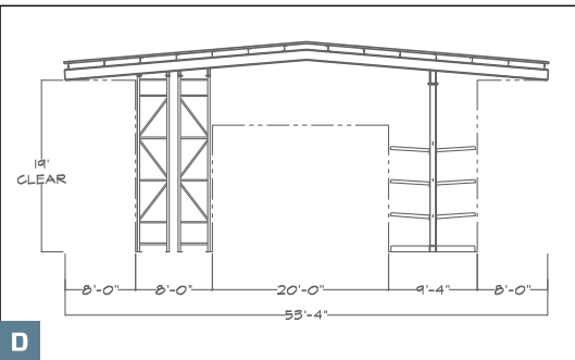
Pallet Rack / Cantilever Building
