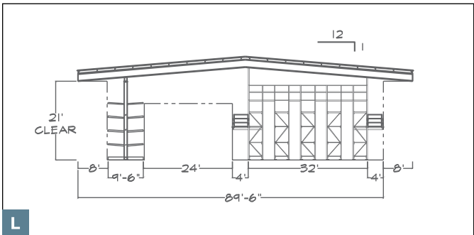
Single-Aisle Power Bin Building
