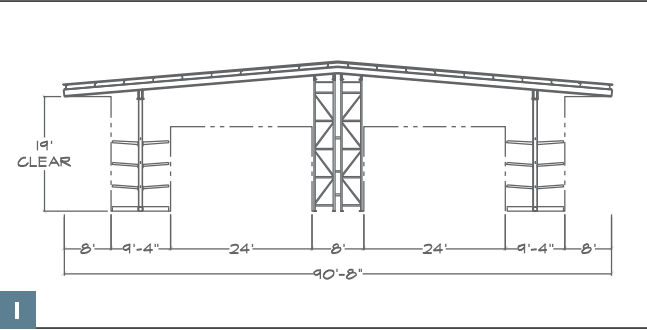
Multi-Purpose Double-Aisle Building
