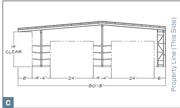
Double-Aisle Property Line Building
