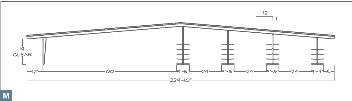
Multi-Purpose Clear Span Drive-Thru Building
