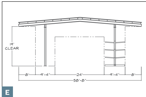
Bulk Storage / Cantilever Building
