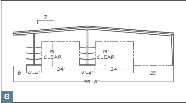
Double-Aisle Cantilever / Bulk Storage Building
