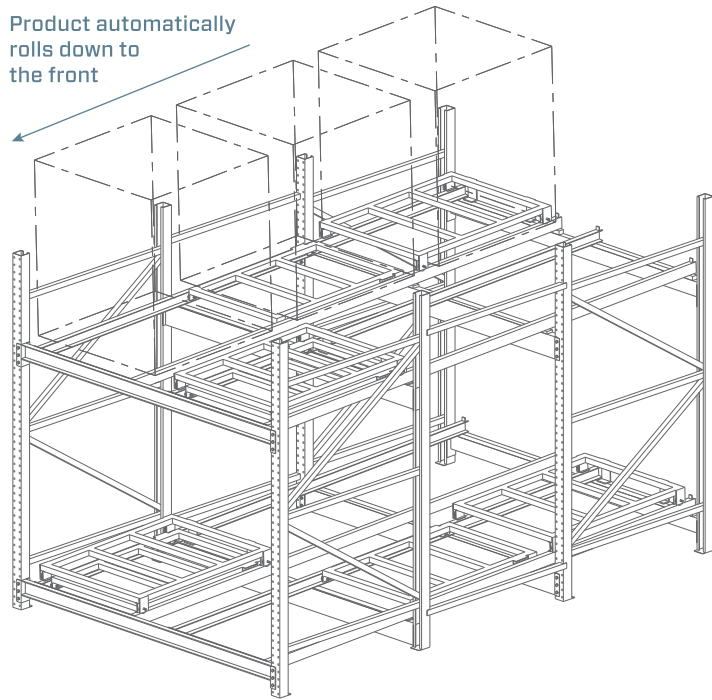
Push-Back Rack
