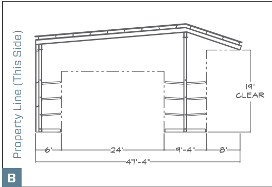
Single-Aisle Property Line Building
