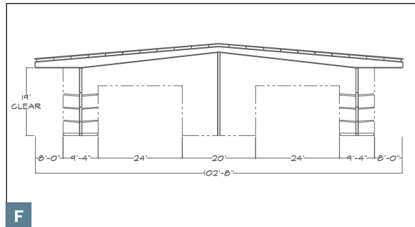
Double-Aisle Cantilever Building
