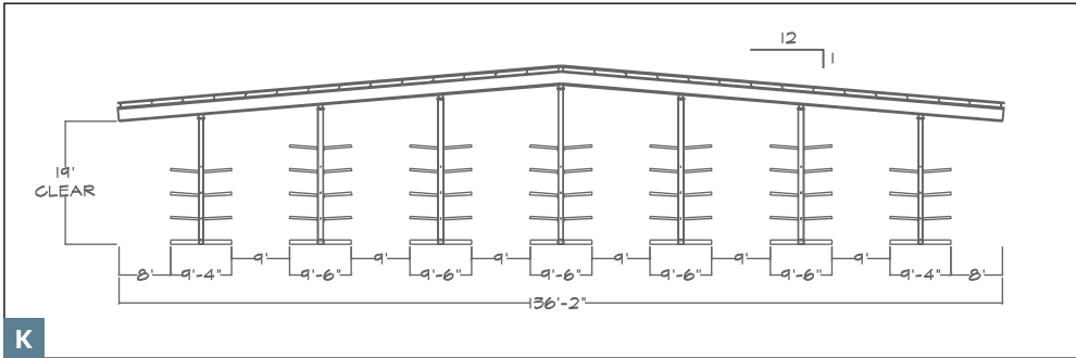
Narrow-Aisle Drive-Thru Building (for side loading forklifts)
