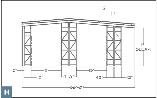
Double-Aisle Pallet Rack Warehouse
