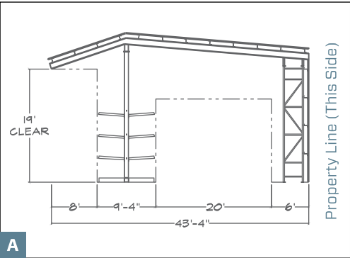
Multi-Purpose Property Line Shed
