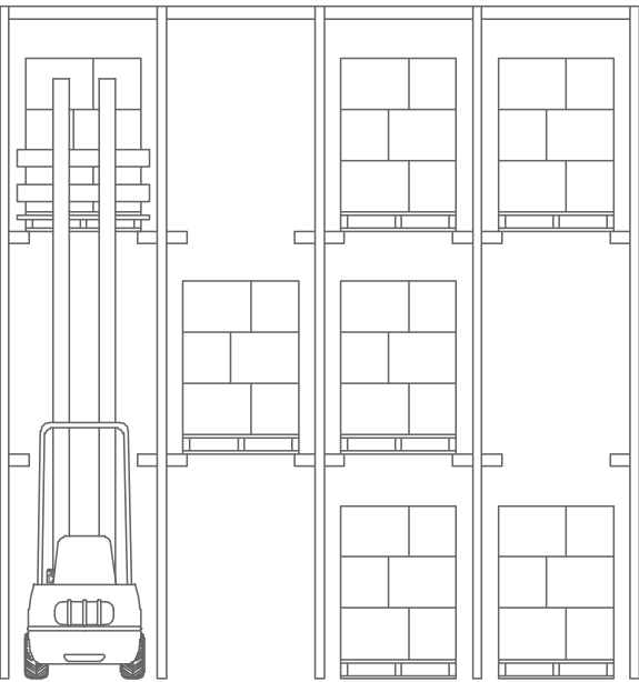
Drive-In Rack
